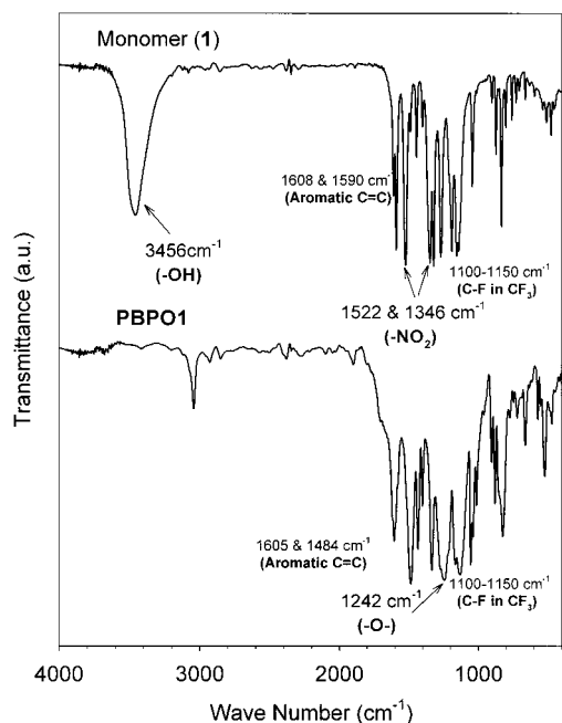
Figure 1. FTIR spectra of monomer 1 (KBr pellet) and polymer PBPO1 (solvent cast thin film).
