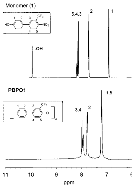
Figure 2. 1 H NMR spectra of monomer 1 (at 25 °C) and polymer PBPO1 (at 100 °C in DMSO- d 6 ).
